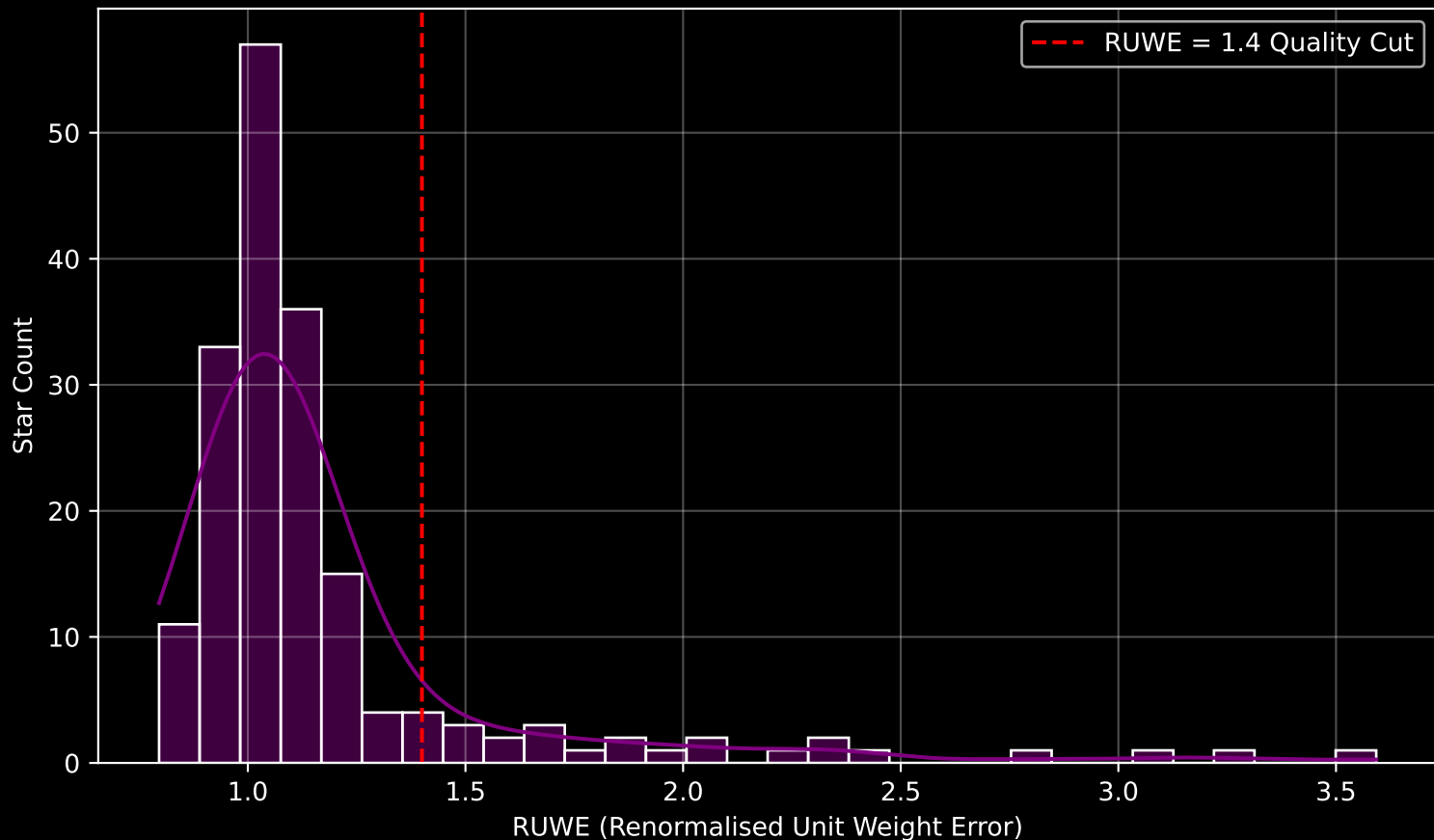
GAPOGEE DR17 Field [182+29_MGA] RUWE Distribution (n= 182)
