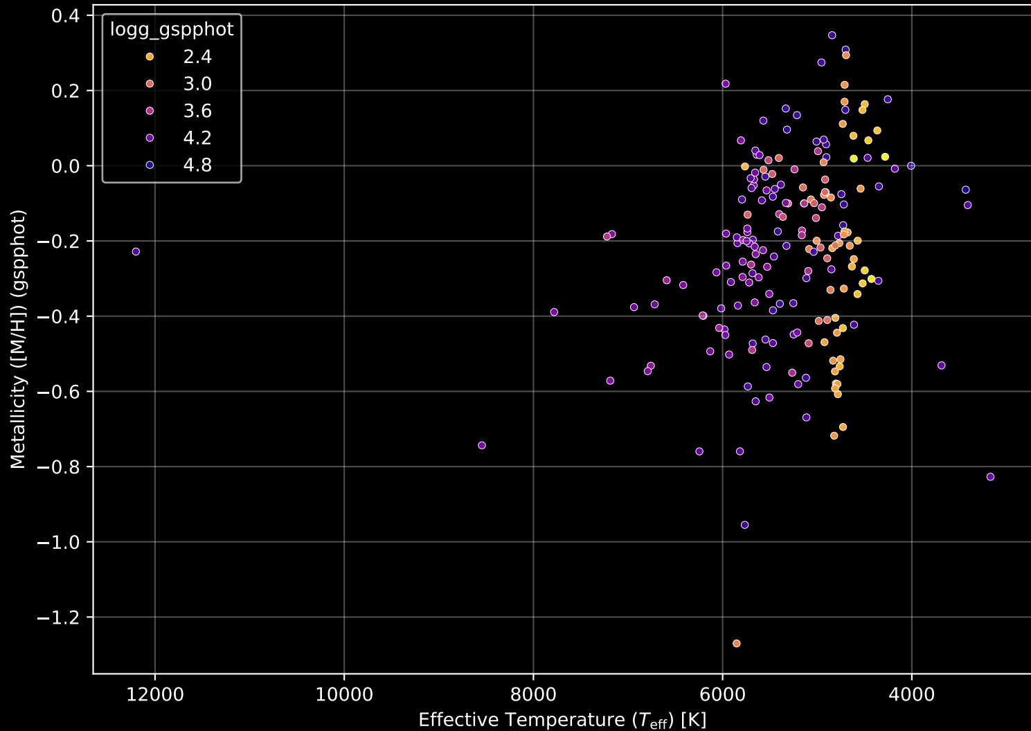
APOGEE DR17 Field: [182+29_MGA] Stellar Population Parameters (n= 193)
