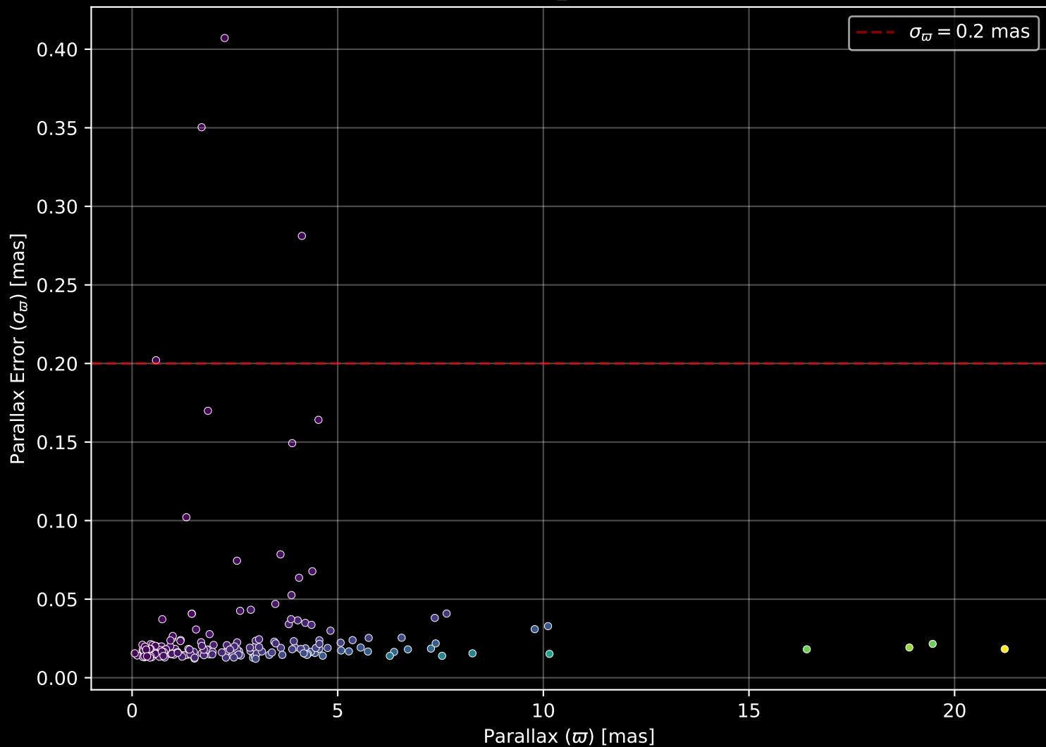
APOGEE DR17 Field: [182+29_MGA] Parallax Quality (n= 193)
