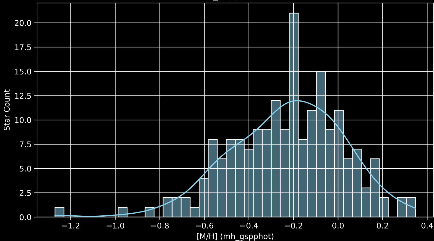
APOGEE DR17 Field: [182+29_MGA [M/H] (mh_gspphot) (n= 193)
