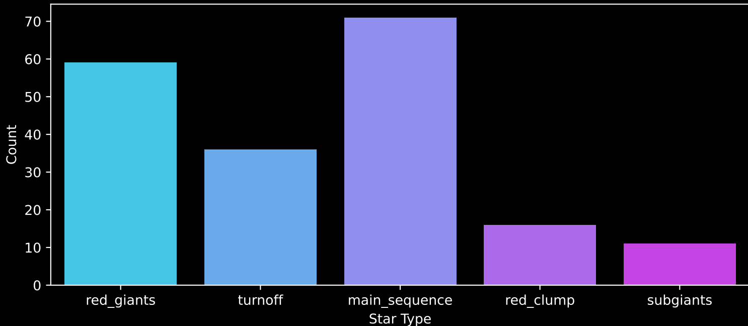
APOGEE DR17 Field: [182+29_MGA] Count plot of Star Type
