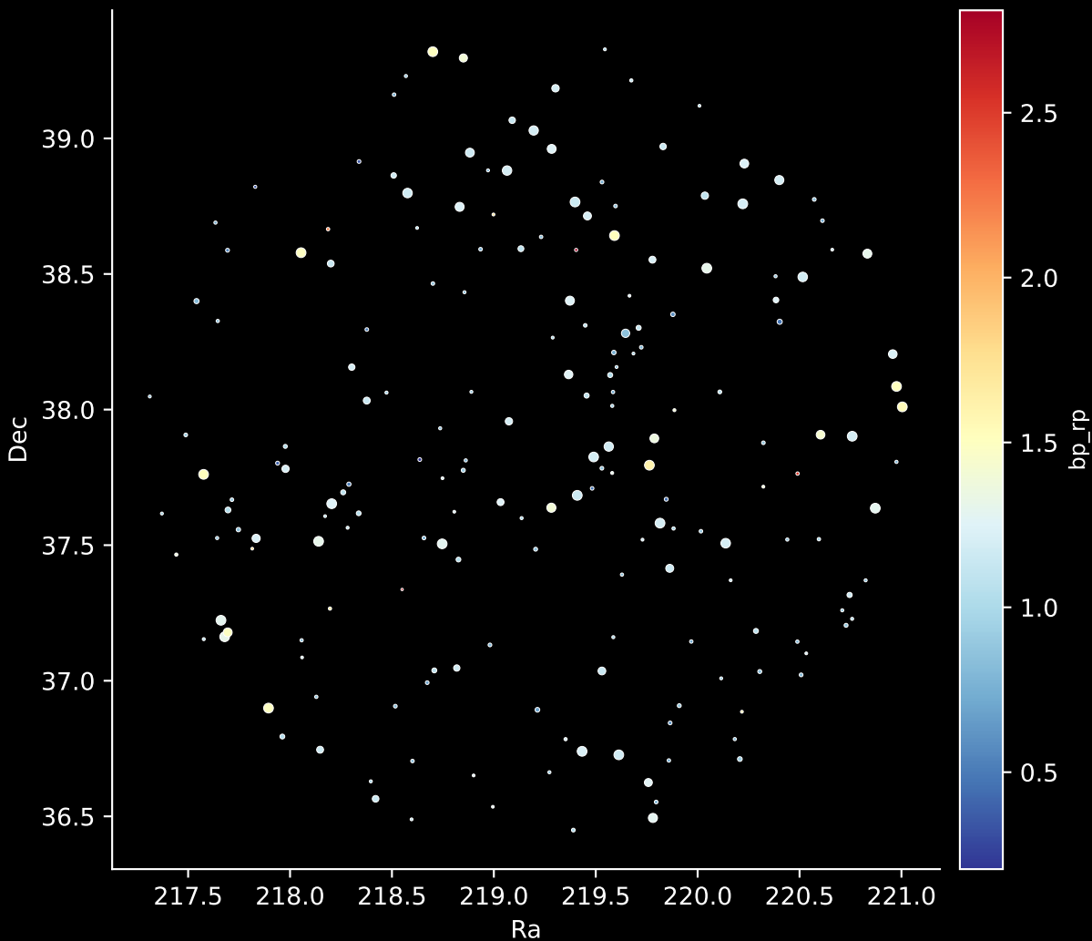
APOGEE DR17 Field: [182+29_MGA] Stars: 193
