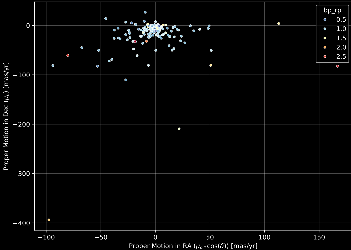
APOGEE DR17 Field: [182+29_MGA] Proper Motion Diagram (n= 193)
